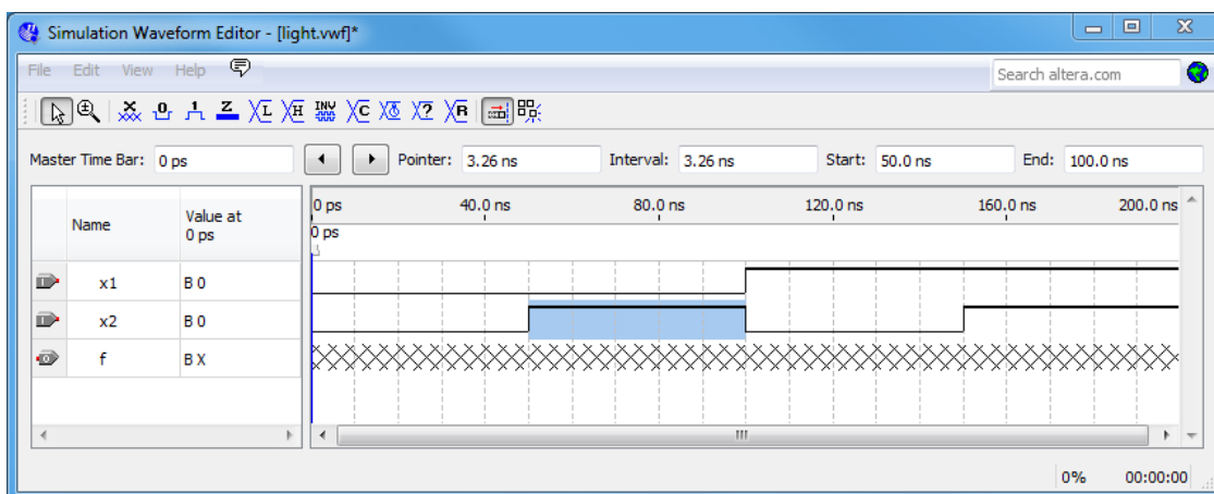
Figure 36. Setting of test values.
